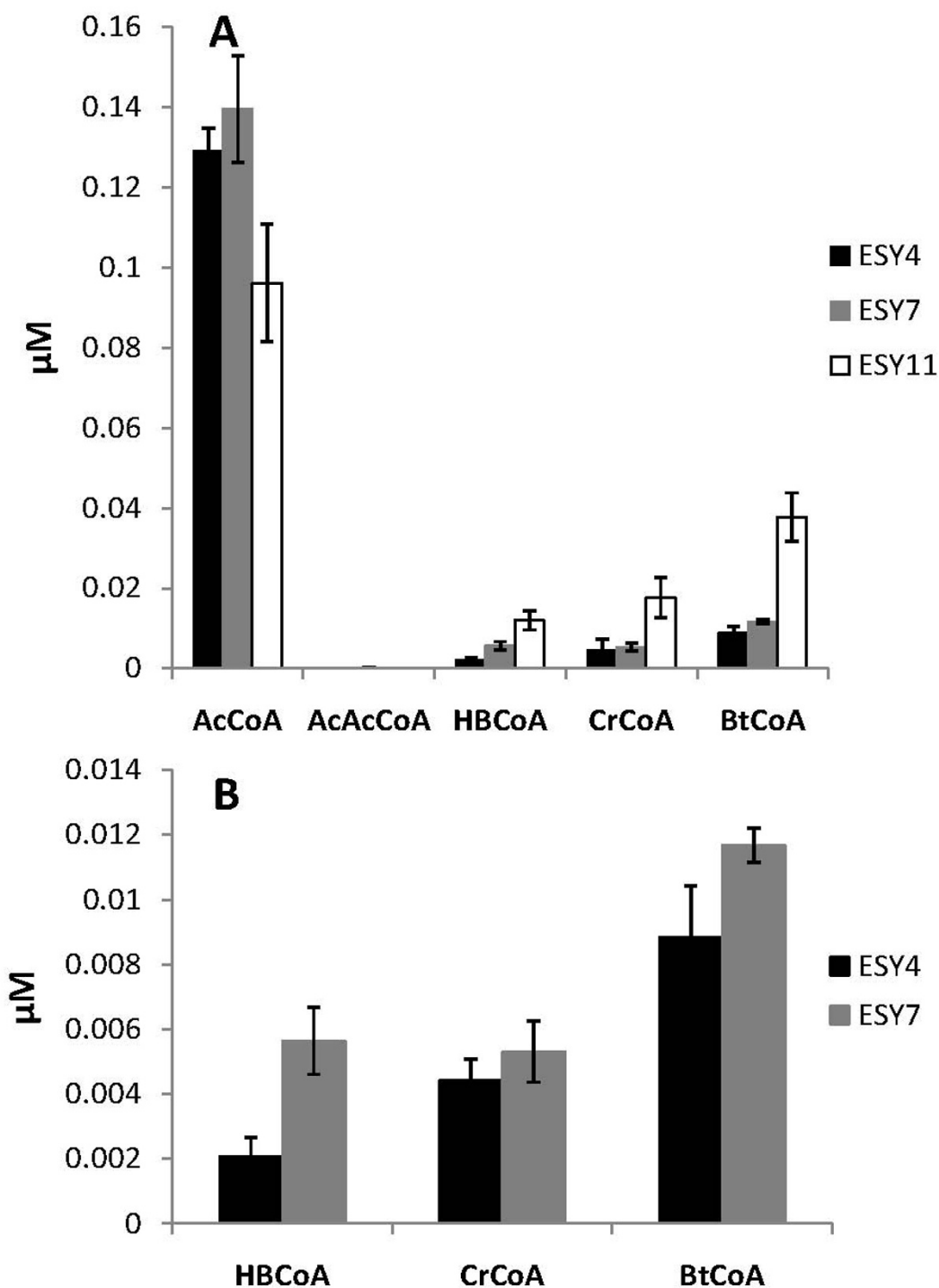
Figure 4 n-Butanol pathway intermediates at 24 h. Bars and strains: black bars, ESY4; gray bars, ESY7; white bars, ESY11. (A) All pathway intermediates in strains ESY4, 7 and 11. (B) HbCoA, CrCoA and BtCoA intermediates in strains ESY4 and ESY7. Levels of AcCoA were similar except for strains ESY11 (A). Levels of 3-hydroxybutyryl-CoA (HbCoA) and butyryl-CoA (BtCoA) were notably higher in ESY7 compared to ESY4, while crotonyl-CoA (CrCoA) was relatively similar in the two strains. Values and error bars represent the mean and standard deviation of triplicate cultures.
