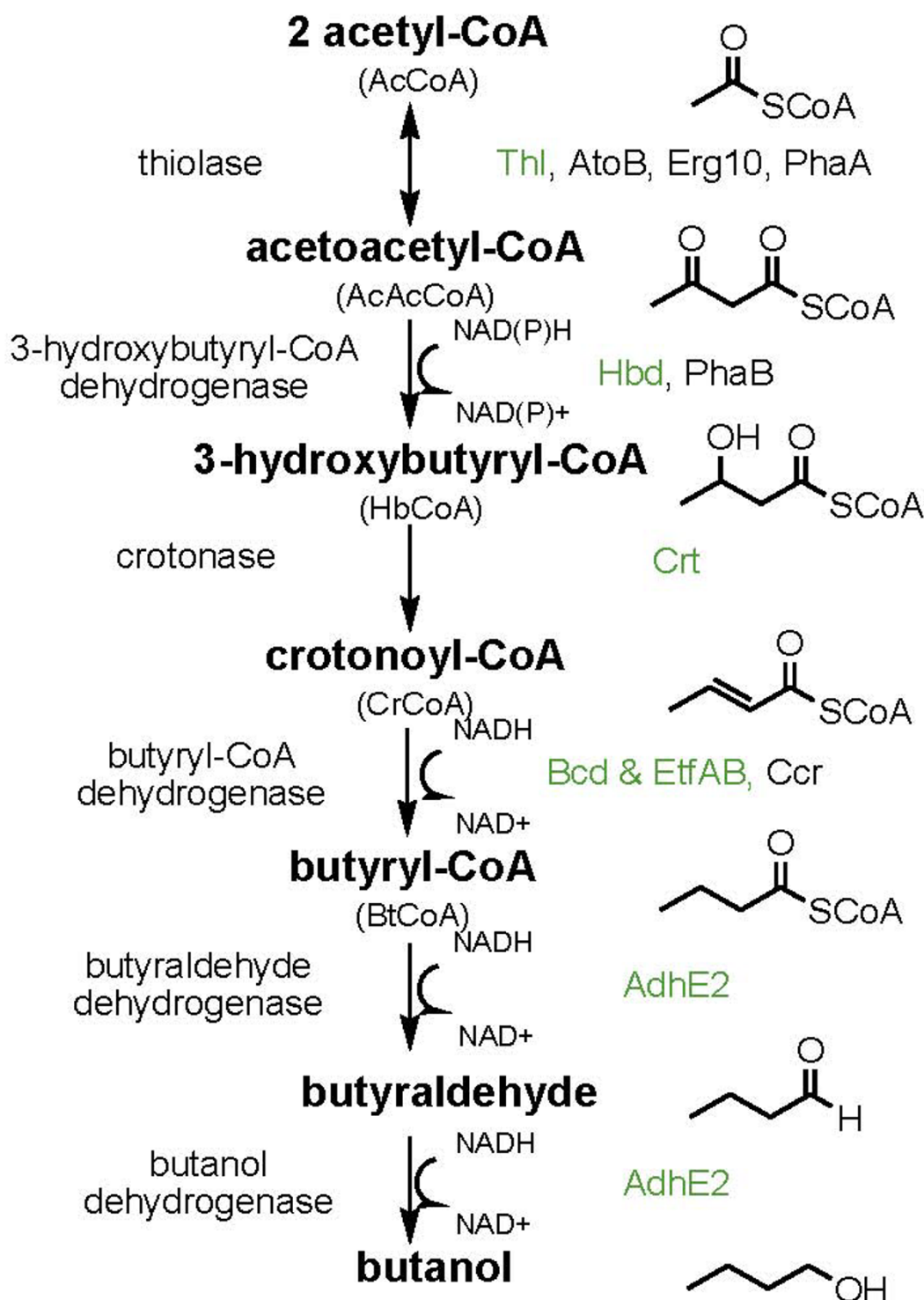
Figure 1 The n-butanol biosynthetic pathway. The enzymes in green are from Clostridium beijerinckii . Enzymes in black are from other organisms: AtoB, Escherichia coli ; Erg10, S. cerevisiae ; PhaA, Ralstonia eutropha ; PhaB, Ralstonia eutropha ; Ccr, Streptomyces collinus . Each enzyme candidate was evaluated in the pathway for n-butanol production (except thl , which is native to Clostridia ).
